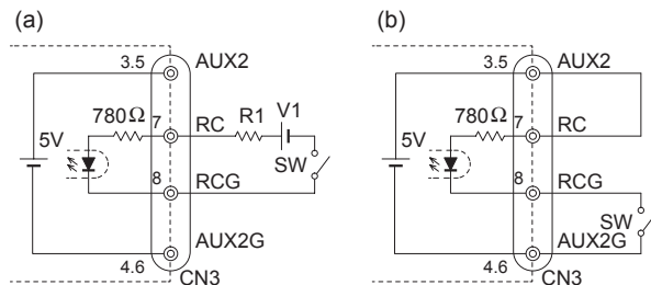
Fig.6.5 RC circuit example
