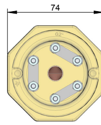
Delta connection D 3x400V
